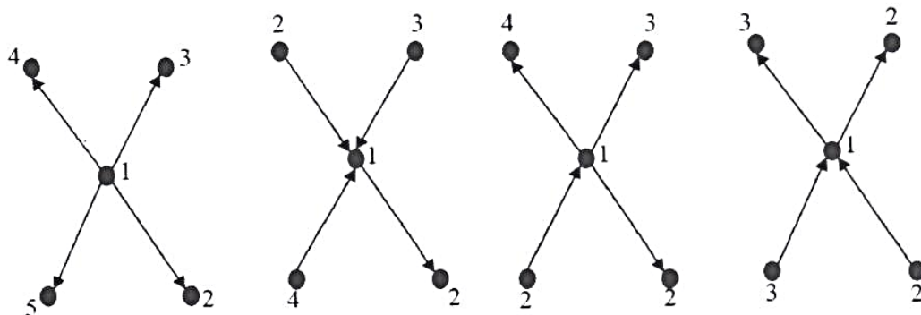
Figure 7: Proper harmonious colorings of S_5 .
