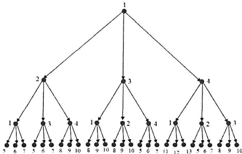
Figure 11: A proper harmonious coloring of complete trinary top-down tree T_3 of level 4.
