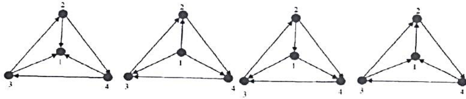
Figure 8: Proper harmonious colorings of unicyclic wheel W_4 .
