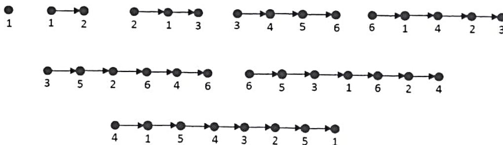
Figure 3: A proper harmonious coloring of union of disjoint unipaths.
