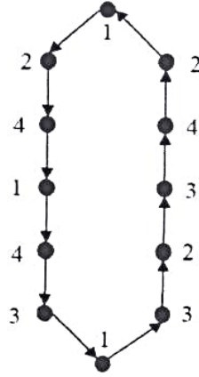
Figure 4: A proper harmonious coloring of unicycle C_{12} .
