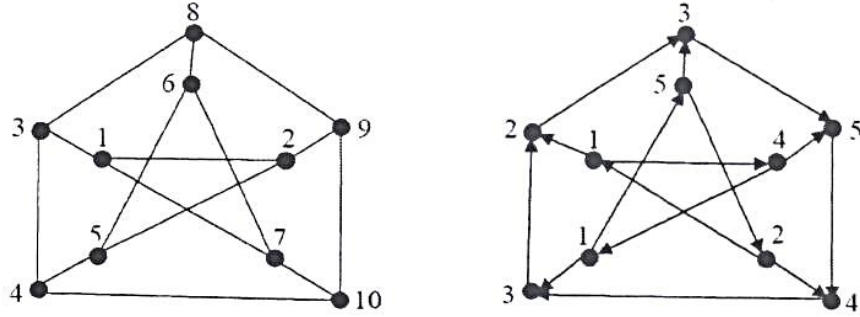
Figure 1: A proper harmonious coloring of Petersen Graph and its oriented graph.
