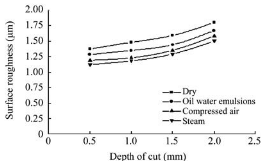
Fig.8 Surface roughness value R_a
