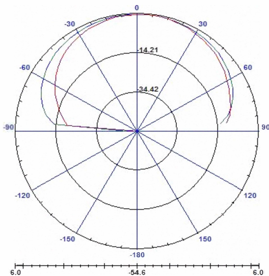
Fig. 5 Radiation pattern of proposed antenna.
