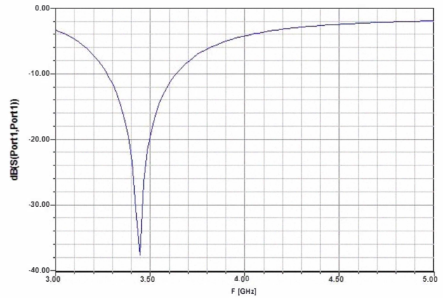
Fig. 2 Return loss vs. Frequency curve for proposed antenna.
