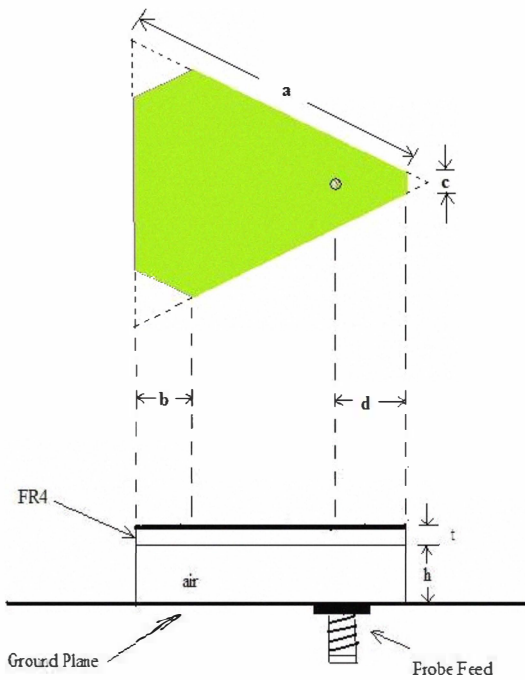
Fig.1 Geometry of proposed triangular microstrip antenna with dimensions a=40.45\text{mm} , b=7.9\text{mm} , c=3.07\text{mm} , d=9\text{mm} , h=6\text{mm} , t=1.6\text{mm} .
