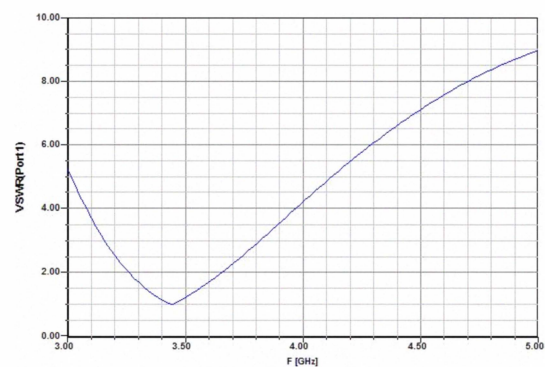
Fig. 4 VSWR vs. Frequency curve for proposed antenna.
