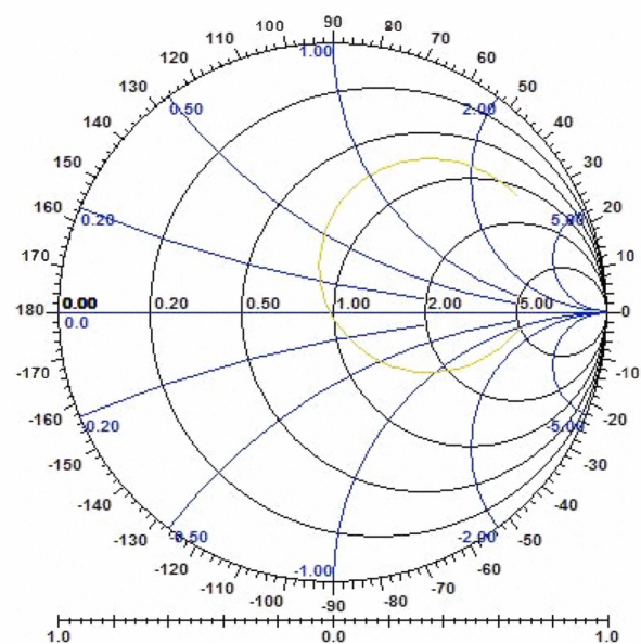
Fig. 3 Input impedance loci using smith chart.
