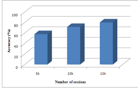
Figure 2. Prediction Accuracy
