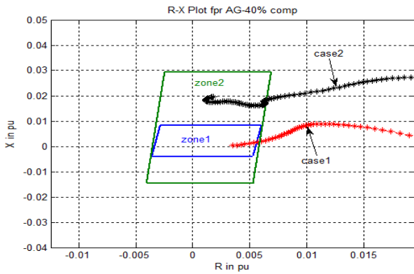
Fig.11.RX plot AG –case 1 and case 2-40% compensation
