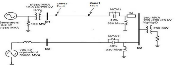
Fig.2. Series compensated transmission system model
