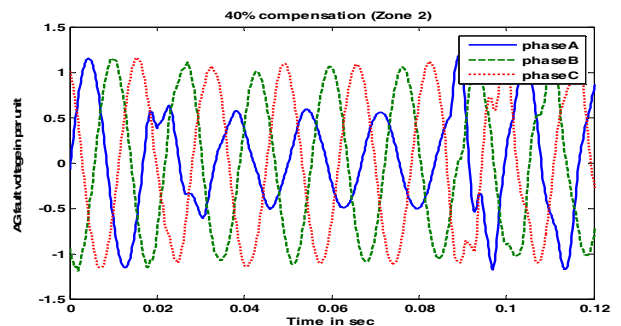
Fig 9 AG fault voltage current for case2 at 40% compensation
