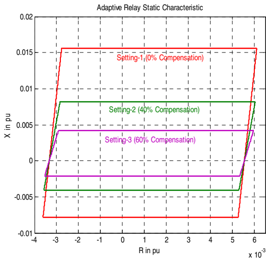
Fig.5 Adaptive Relay characteristic for Zone 1 w.r.t. level of compensation
