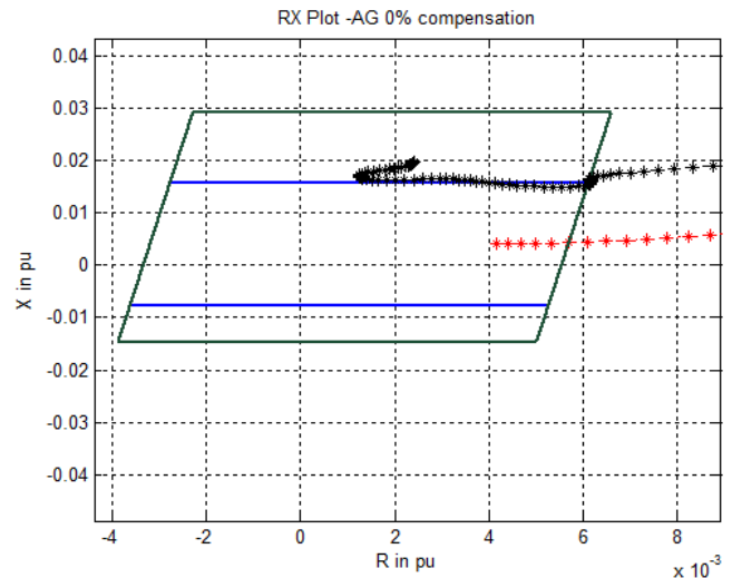
Fig.15.RX plot for case1 and case2 at 0% compensation
