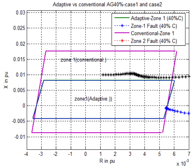
Fig.16 R X plot for Adaptive relay Vs Conventional relay for case1 and case2 at 40 % compensation
