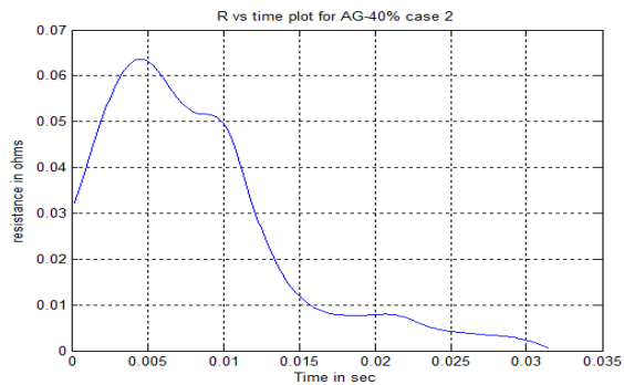
Fig.13. R Vs T plot for AG-case2 at 40% compensation
