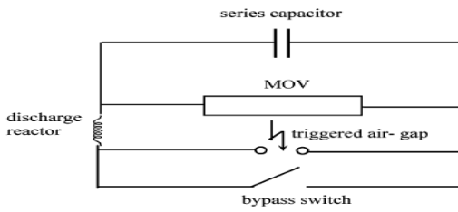
Fig.3 MOV protected series capacitor.
