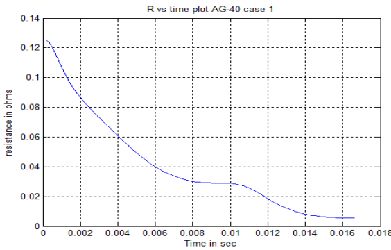
Fig.12 R Vs T plot for case 1 at 40% compensation
