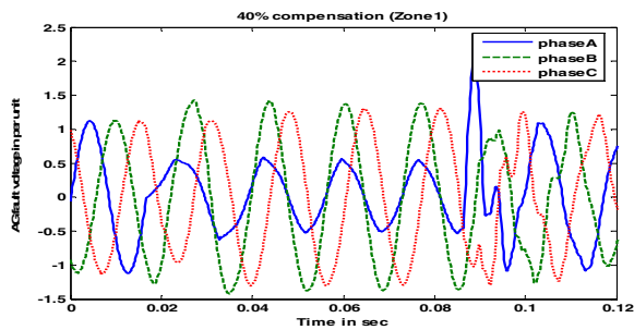
Fig7. AG fault voltage for case1 at 40% compensation
