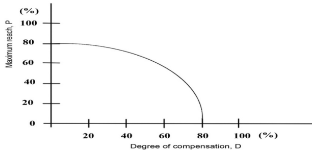
Fig. 4. First zone maximum reach as a function of the degree of compensation "D", the degree of compensation of the line is given as
