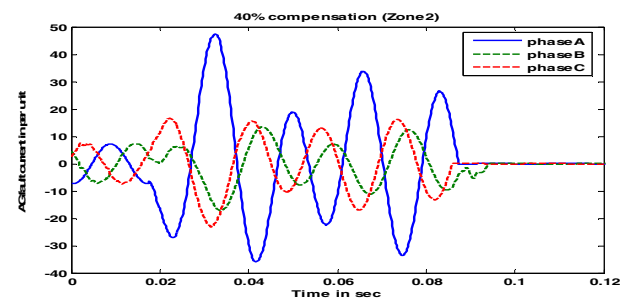
Fig.10 .AG fault current-case2-40% compensation
