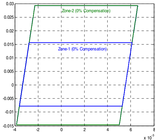
Fig.6. zone1 and zone2.of conventional Relay (0 % compensation) characteristic,
